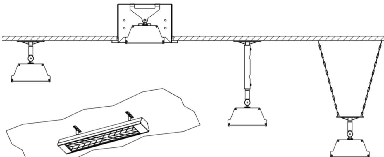
Standard Ceiling Bracket
