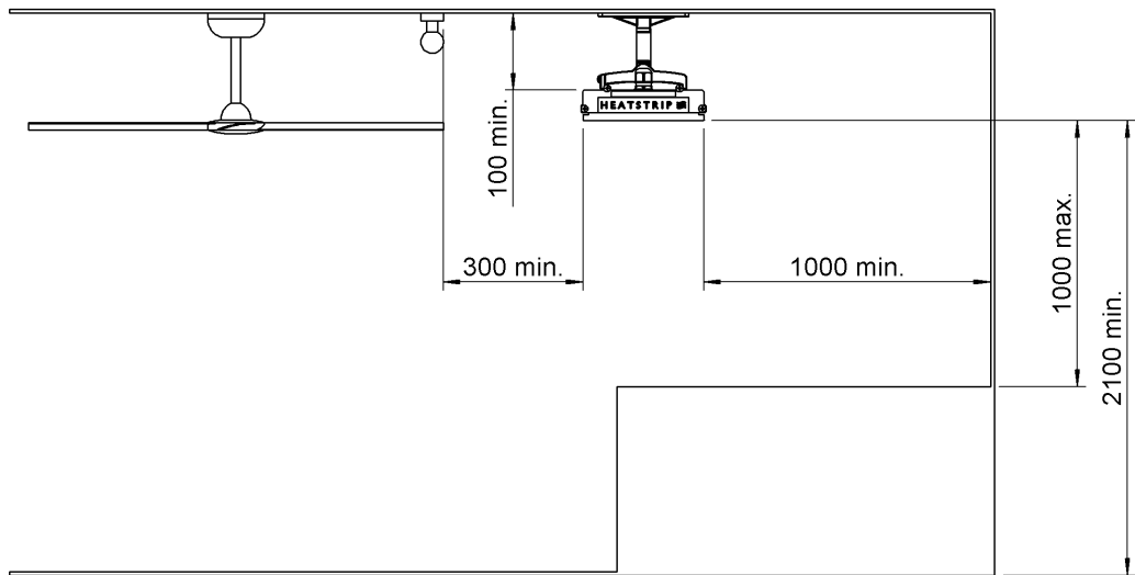
Ceiling Installation
